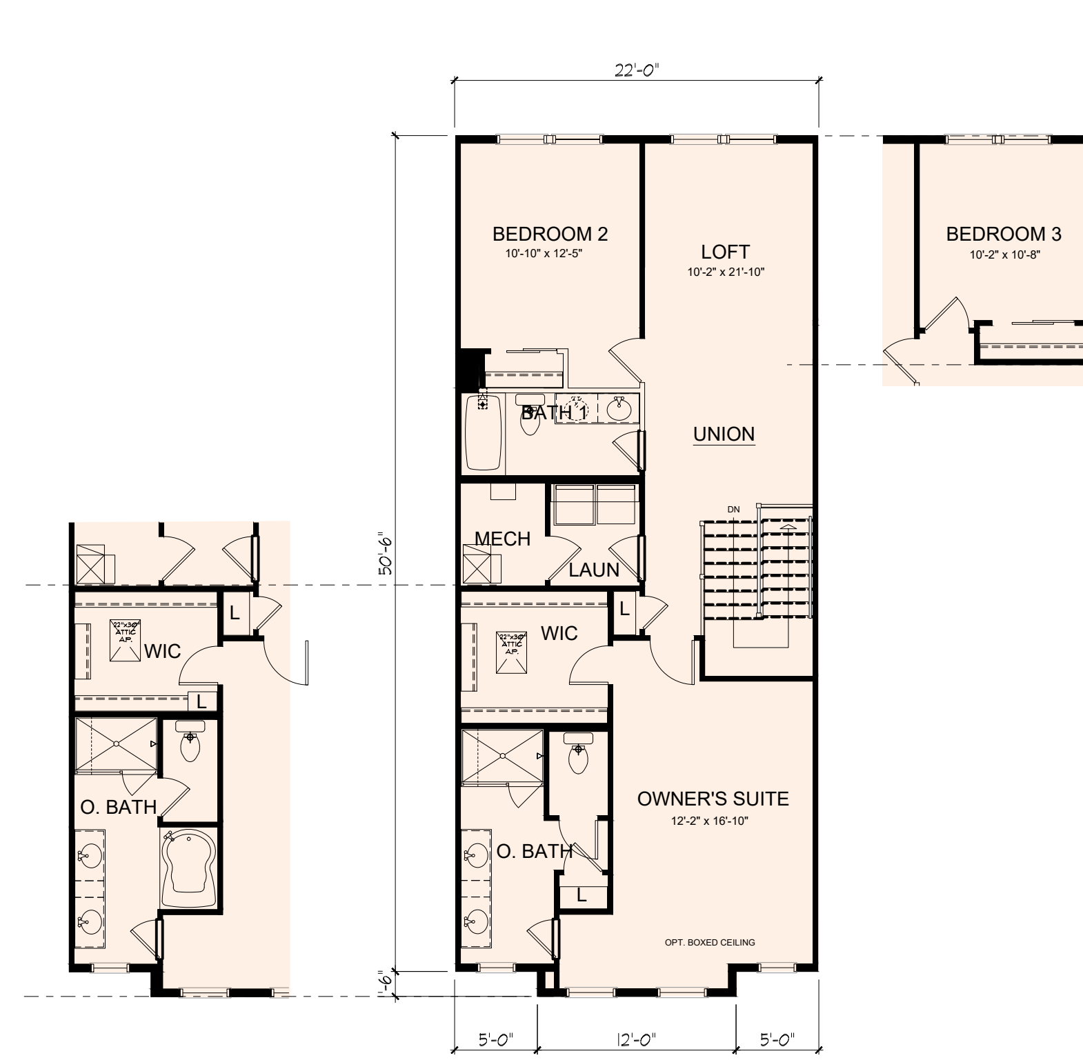
3rd FL PLAN UNION 1/8" = 1'-0"
