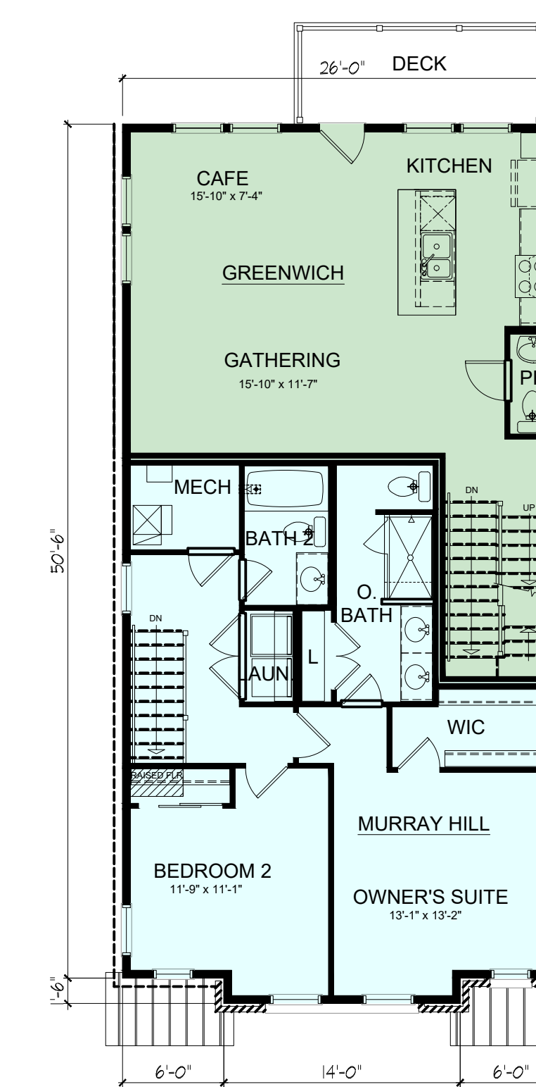
2nd FL PLAN MURRAY HILL / GREENWICH 1/8" = 1'-0"
