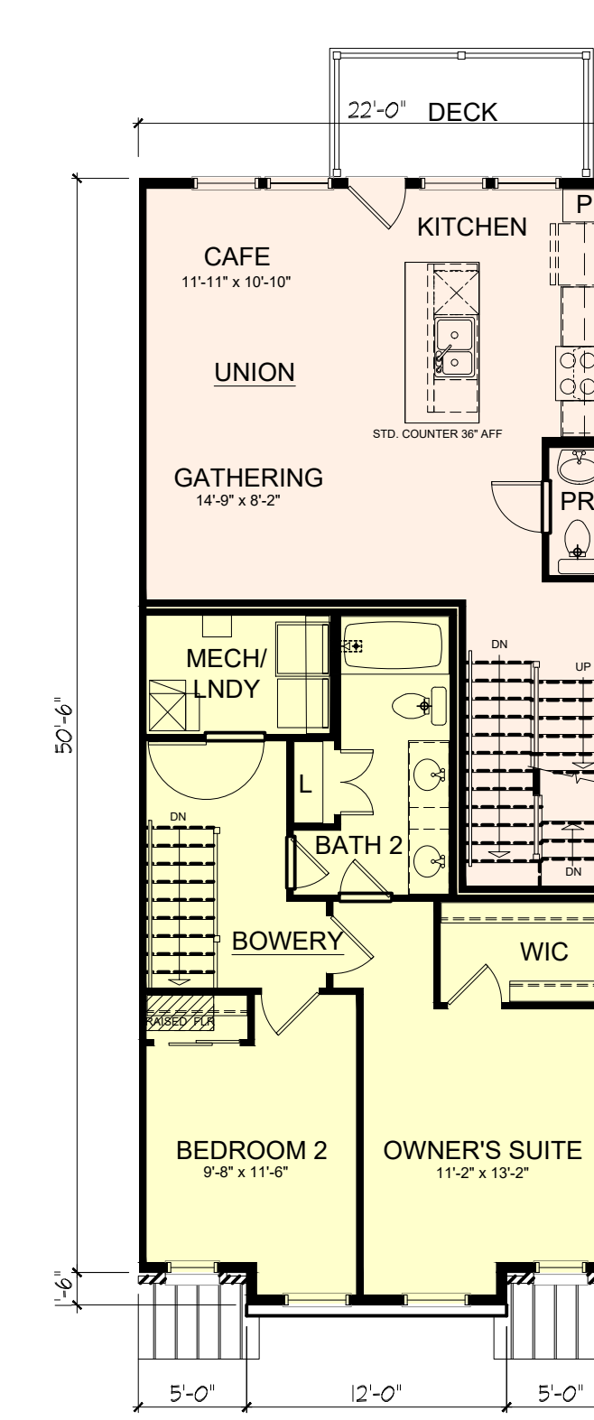
2nd FL PLAN UNION / BOWERY 1/8" = 1'-0"
