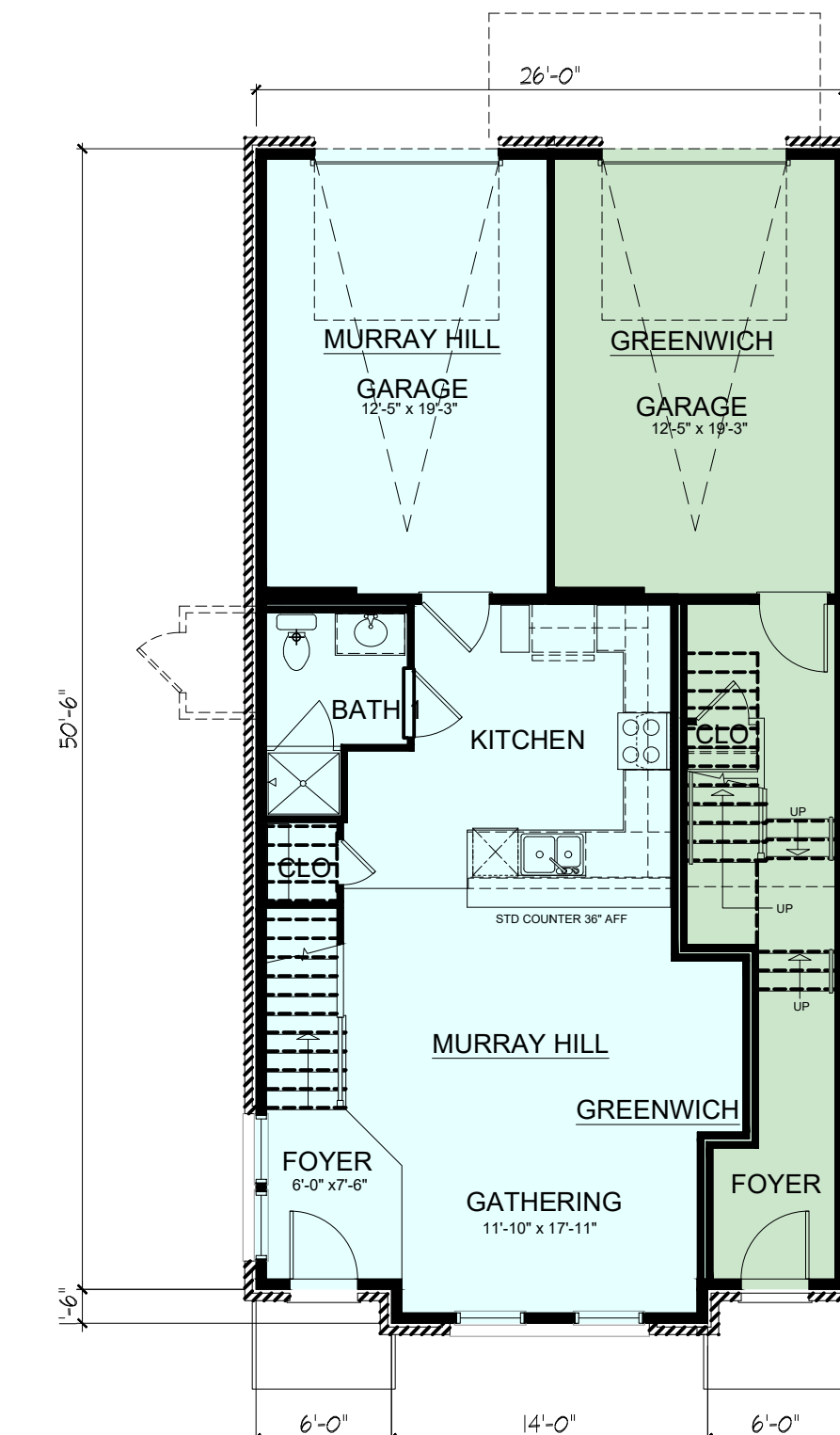
1st FL PLAN MURRAY HILL / GREENWICH 1/8" = 1'-0"
